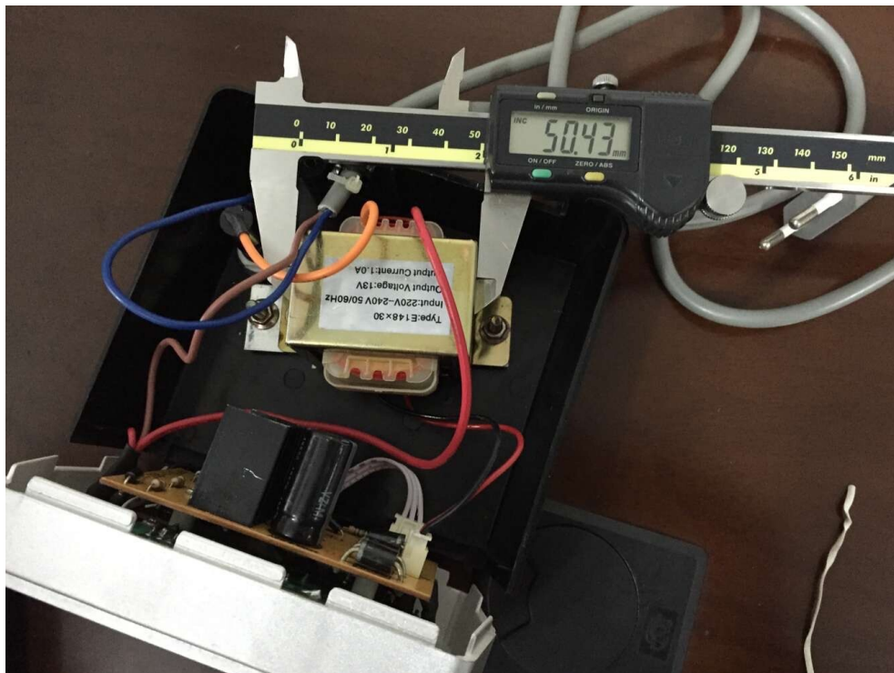
The smaller the transformer, the less the cost, the power smaller.
